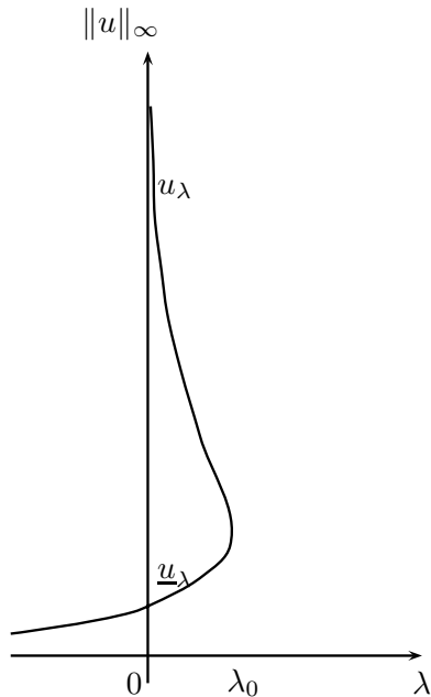
FIGURE 1. Bifurcation diagram for solutions of problem (1.4)
